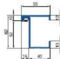
Blockzarge 62/55
