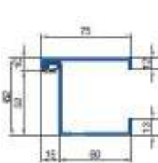
Blockzarge 62/75
