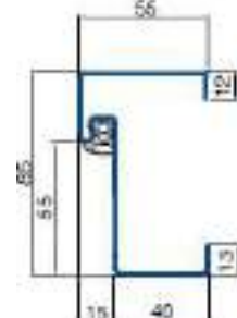
Blockzarge 85/55 Standard
